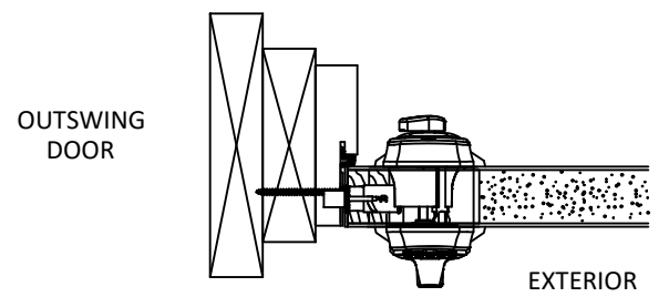
SECTION A-A DEADBOLT WITH FUSION BOLT PLATFORM
