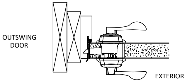
SECTION B-B SCHLAGE F-SERIES CYLINDRICAL LATCH
