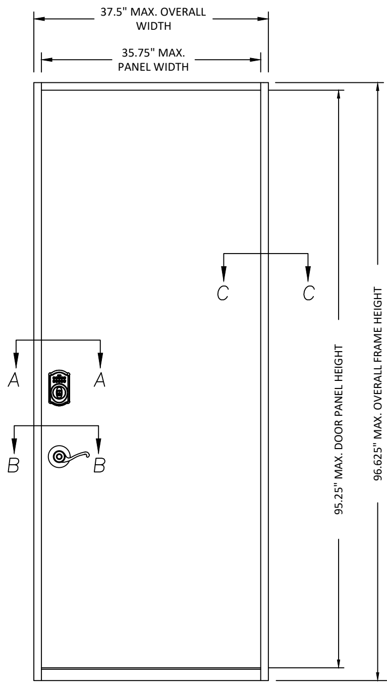
EXTERIOR ELEVATION SINGLE FLUSH/OPQAUE INSWING/OUTSWING (DOOR UNDER SEPARATE APPROVAL)
