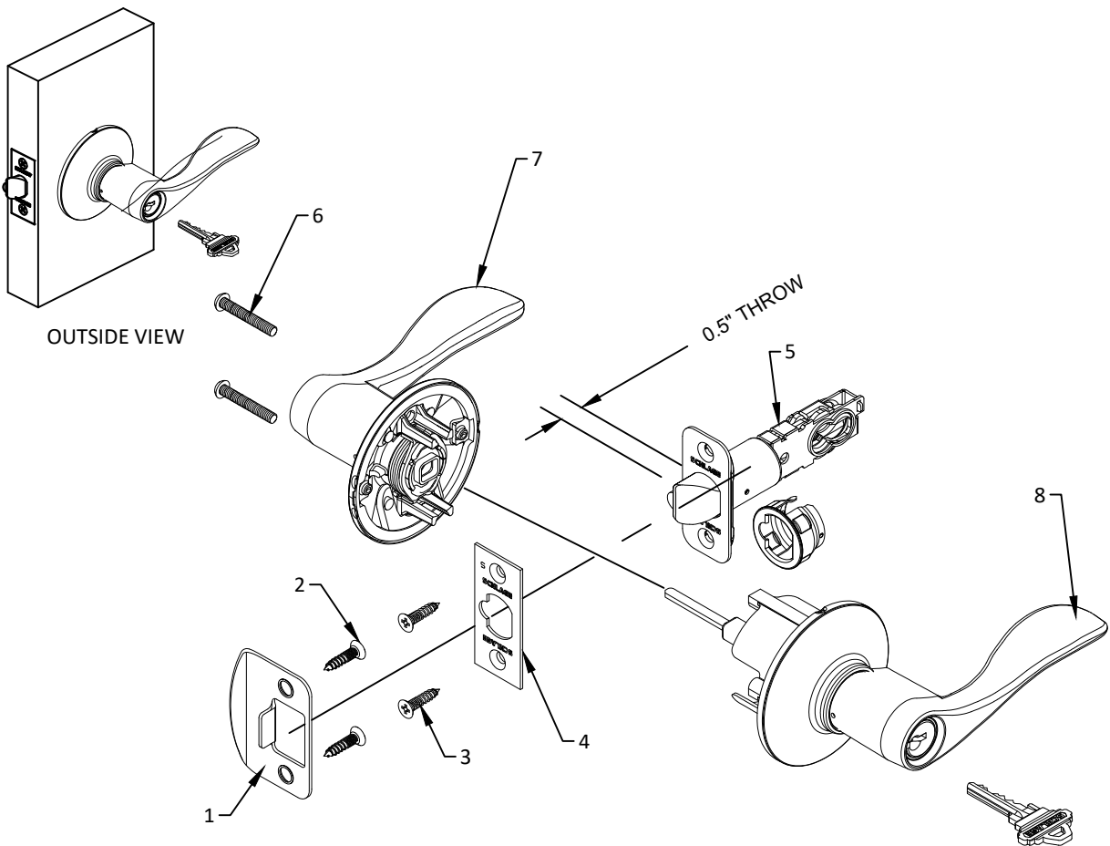
SCHLAGE F/FA/FE/FC-SERIES CYLINDRICAL LOCK TO BE USED WITH: SCHLAGE B-SERIES OR BE-SERIES DEADLOCK LOCKS MAY HAVE KNOB, LEVEL OR GRIP HANDLESET
