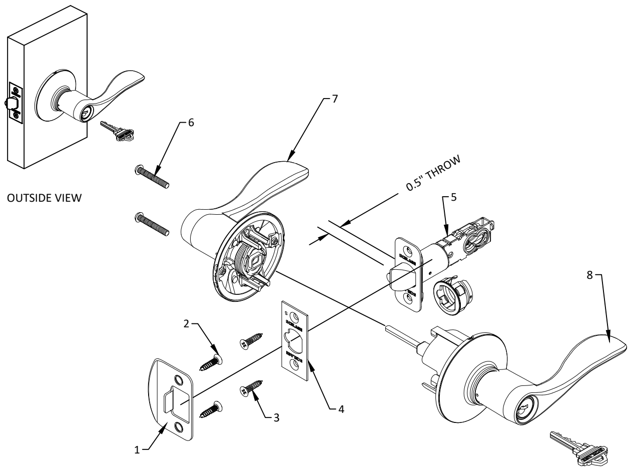
SCHLAGE F/FA/FE/FC-SERIES CYLINDRICAL LOCK TO BE USED WITH: SCHLAGE B-SERIES OR BE-SERIES DEADLOCK LOCKS MAY HAVE KNOB, LEVEL OR GRIP HANDLESET
