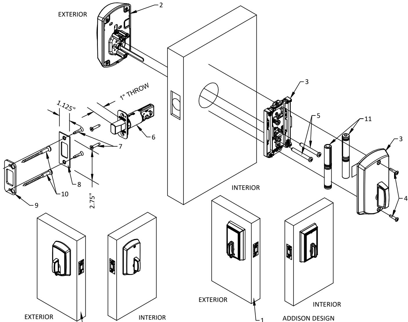
SCHLAGE BE467F SERIES CYLINDRICAL DEADLOCK TO BE USED WITH SCHLAGE F/FA/FE/FC-SERIES LOCKS LOCKS MAY HAVE KNOB, LEVER OR GRIP HANDLESET
