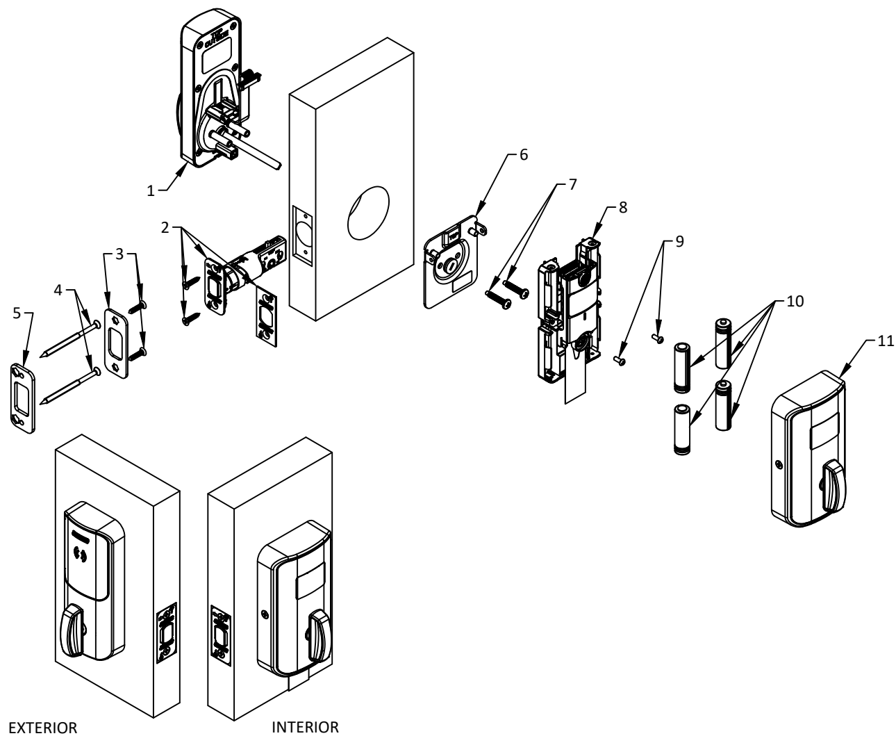
SCHLAGE XE360-DB SERIES CYLINDRICAL DEADLOCK TO BE USED WITH SCHLAGE F/FA/FE/FC-SERIES LOCKS LOCKS MAY HAVE KNOB, LEVER OR GRIP HANDLESET
