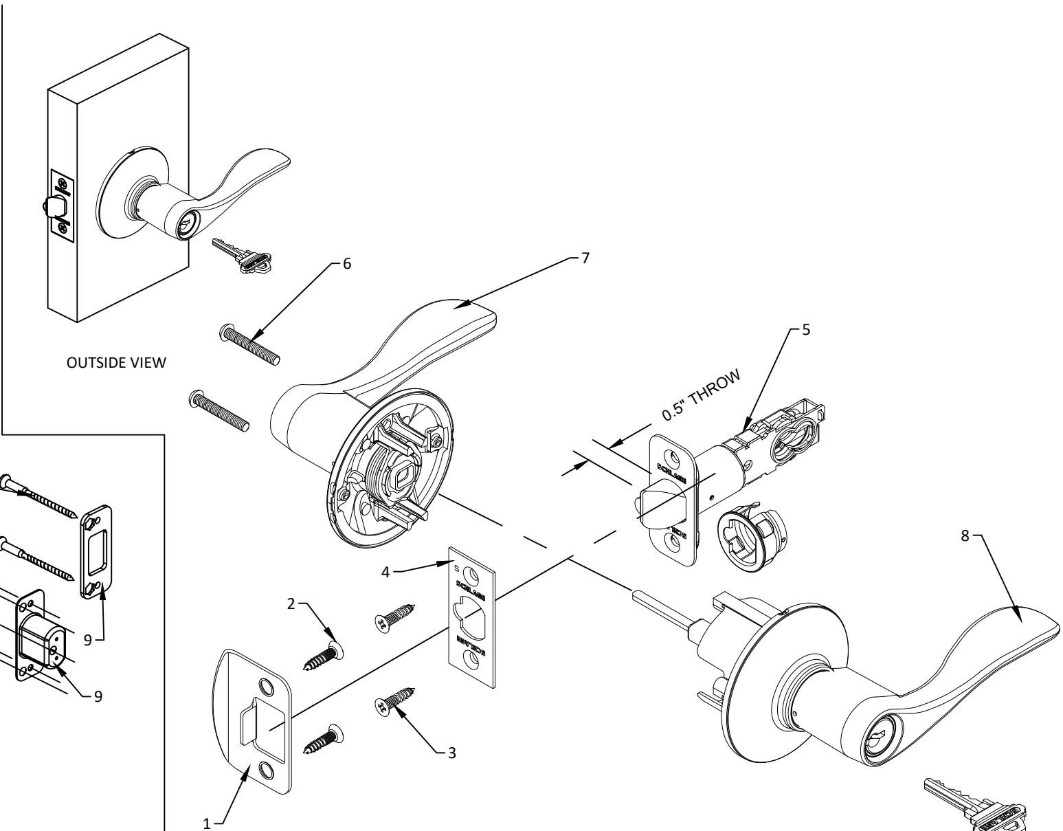
SCHLAGE F/FA/FE/FC-SERIES CYLINDRICAL LOCK TO BE USED WITH: SCHLAGE B-SERIES OR BE-SERIES DEADLOCKS LOCKS MAY HAVE KNOB, LEVEL OR GRIP HANDLESET
